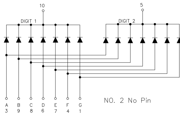
CSOD-30201 is Common Cathode
